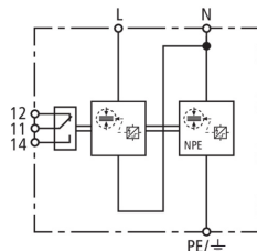
Basic circuit diagram DVA CSP 1P 50 S FM
