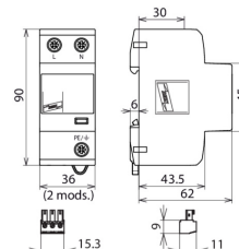
Dimension drawing DVA CSP 1P 50 S FM
